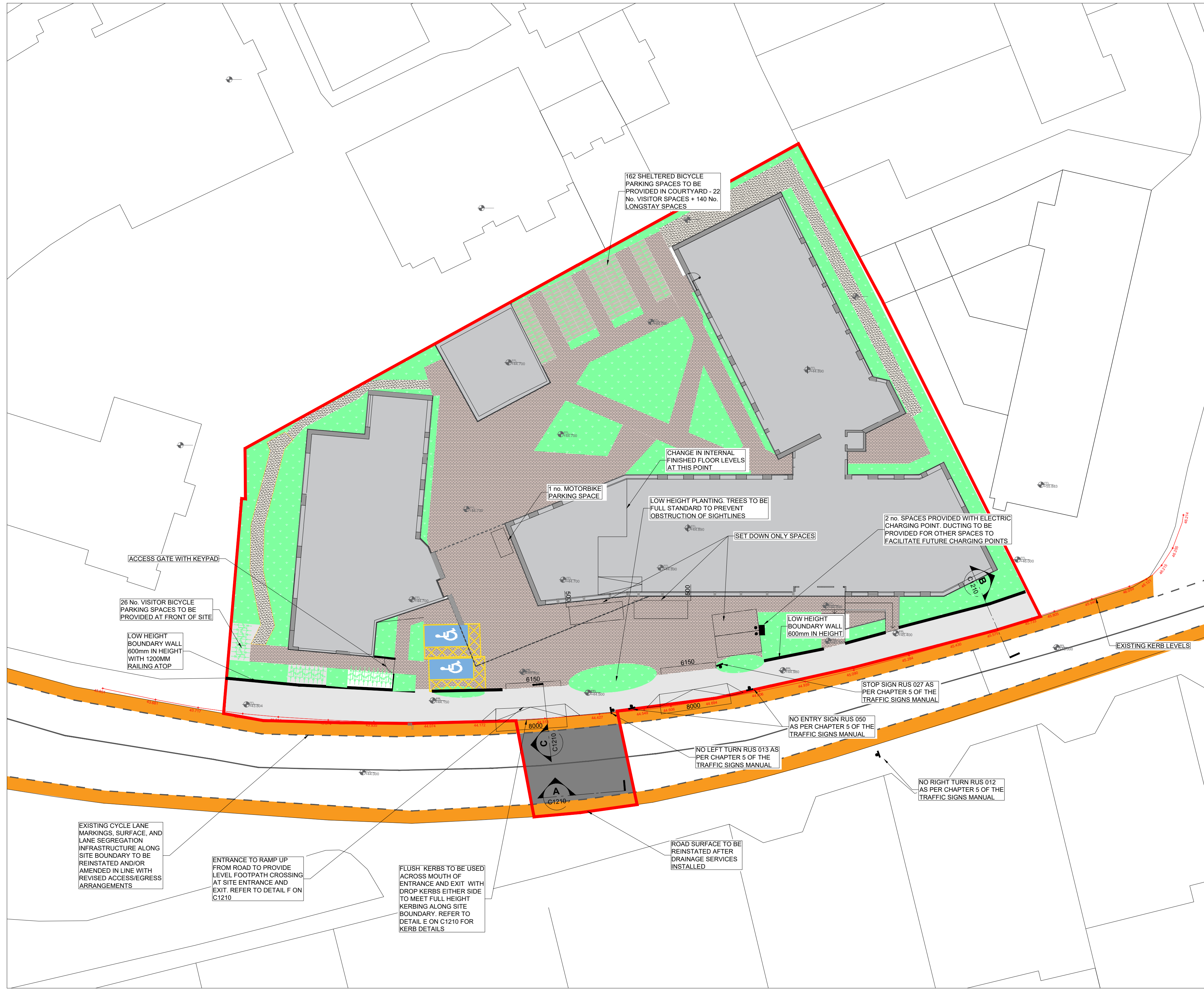
LAYOUT SCALE @ A1: 1:250 SCALE @ A3: 1:500
